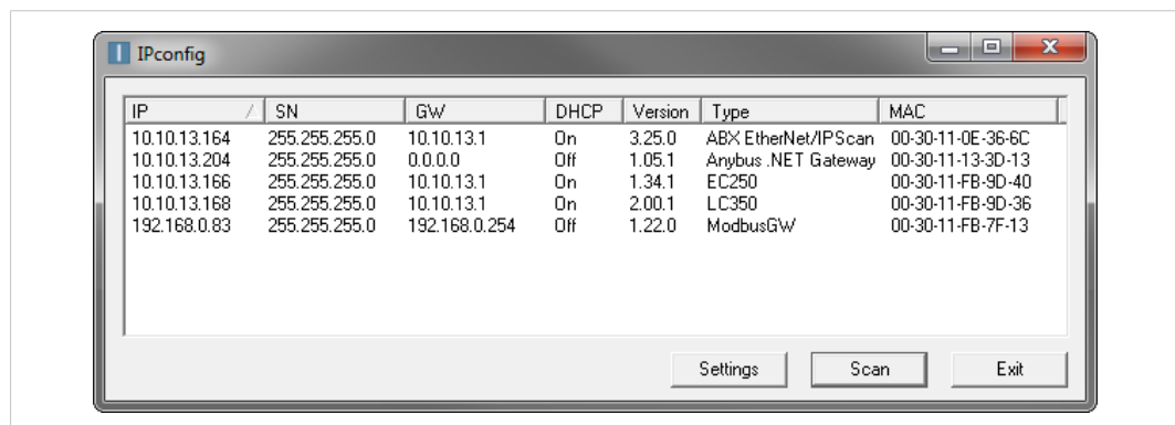
Fig. 33 IPconfig main window
