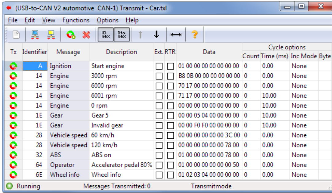
Figure 5.31: Transmit module CAN
