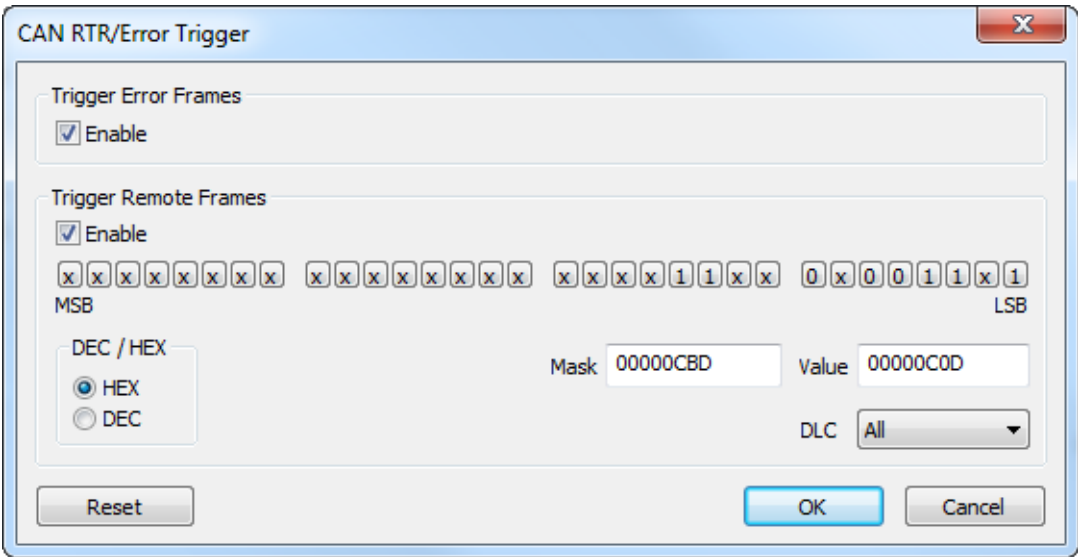
Figure 5.43: CAN RTR/error trigger
