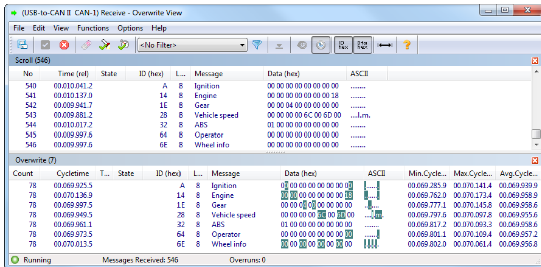
Figure 5.25: Receive module
